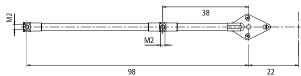
Probe arm FTM-HR-L038*098 - M2*M2
